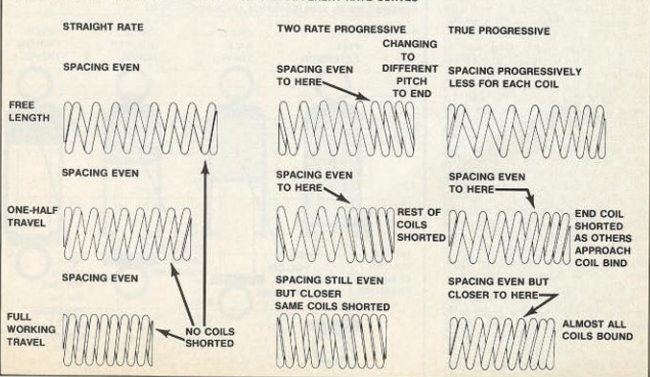
FIGURE TWO HOW VARIOUS TYPES OF COIL SPACING RESULTS IN DIFFERENT RATE CURVES
