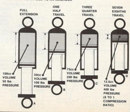
FIGURE THREE BOYLE'S LAW AS APPLIED TO AN AIRSHOCK
