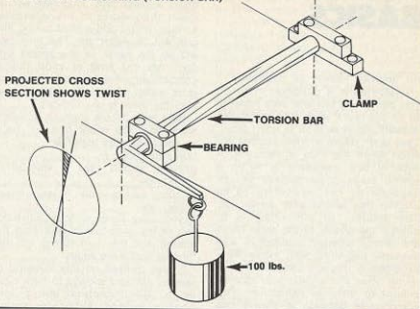
FIGURE ONE UNWRAPPED COIL SPRING (TORSION BAR)
